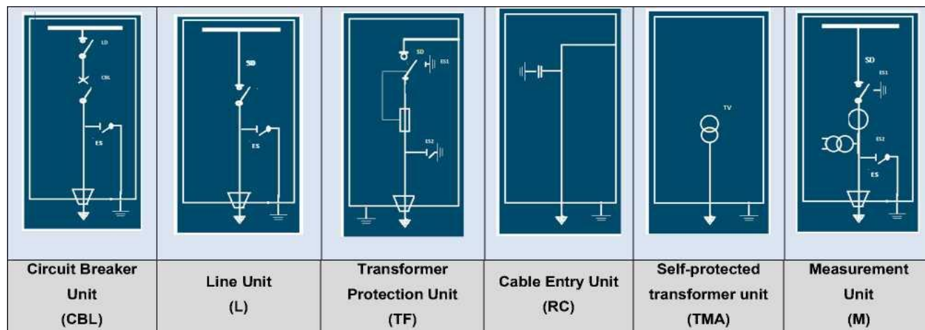
Figure 1 - Functional schemes
